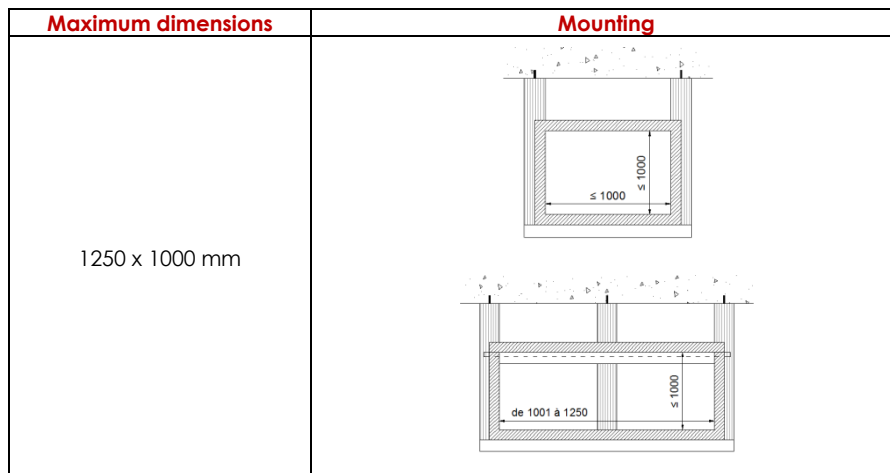
Fig. 4: Figure 2.2.4.3 : Horizontal duct composed of GEOFLAM® F Light fire protective boards
