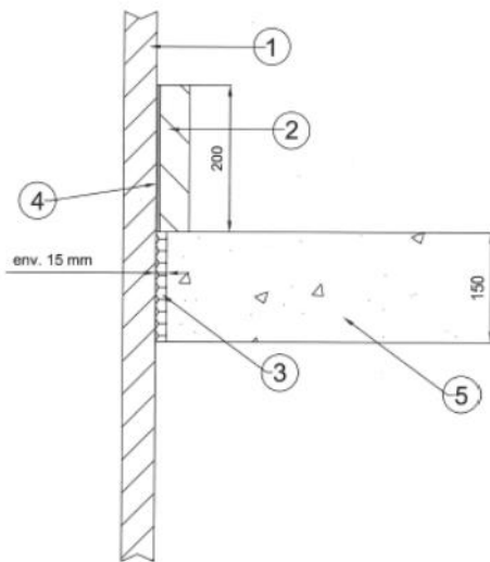
Fig. 8: Figure 2.3.5.1: Vertical duct composed of GEOFLAM® F Light fire protective boards
