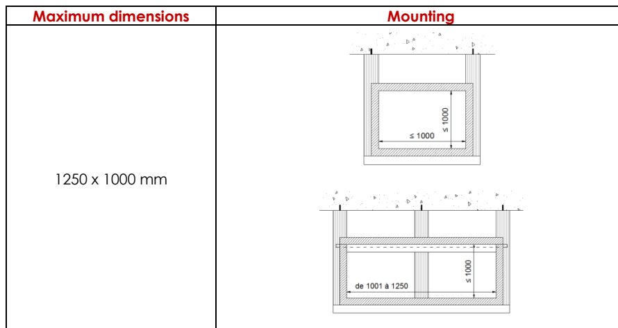
Fig. 7: Figure 2.3.4.3 : Horizontal duct composed of GEOFLAM® F Light fire protective boards
